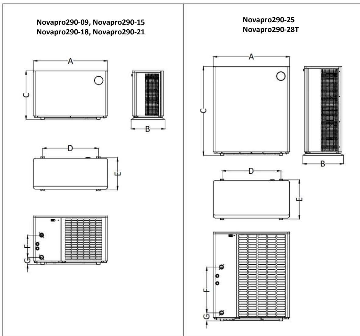
Dimension Indication (unit: mm)
